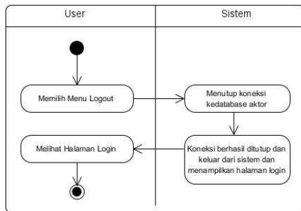
Gambar 7. Activity Diagram Logout
