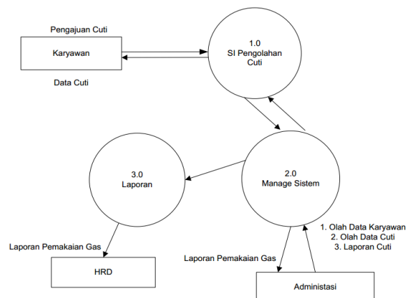
Gambar 7. Diagram Level 0
