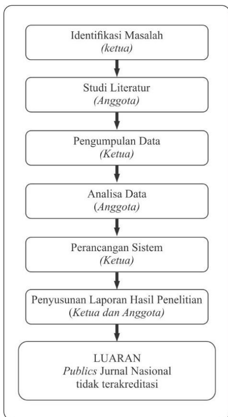
Gambar 2. Alur Penelitian
